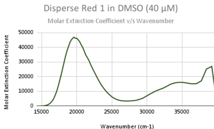
Fig. 3(j) Variation of \epsilon with wavenumber for given concentration of Disperse Red 1
