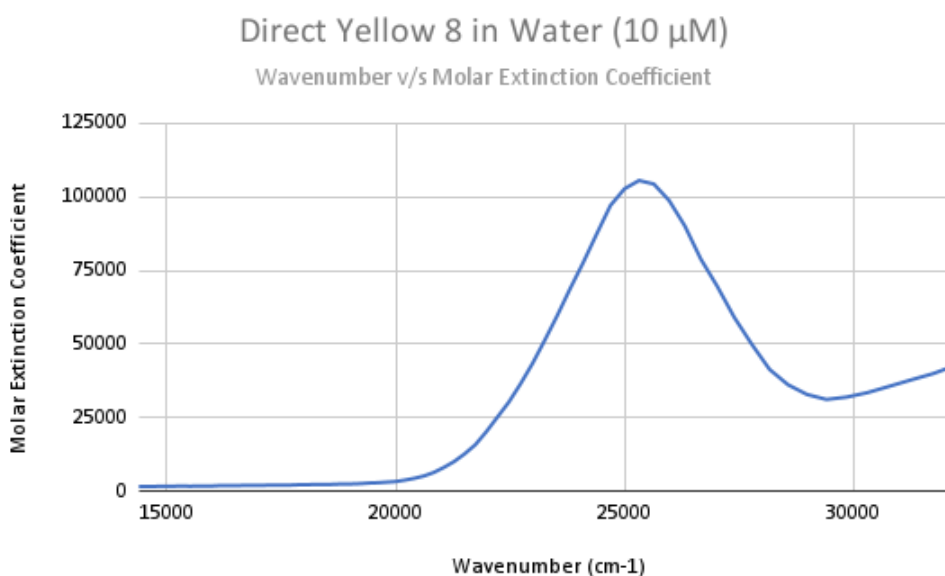
Fig. 3(b) Variation of \epsilon with wavenumber for given concentration of Direct Yellow 8
