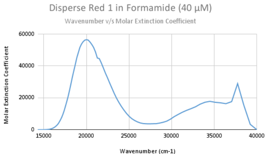
Fig. 3(h) Variation of \epsilon with wavenumber for given concentration of Disperse Red 1
