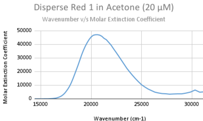
Fig. 3(f) Variation of \epsilon with wavenumber for given concentration of Disperse Red 1
