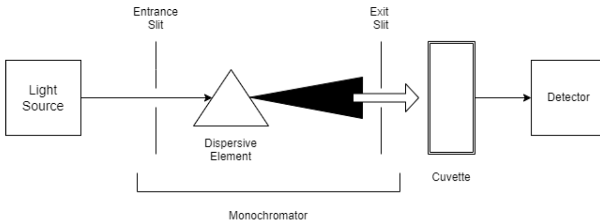
Fig. 2 Spectrophotometer
